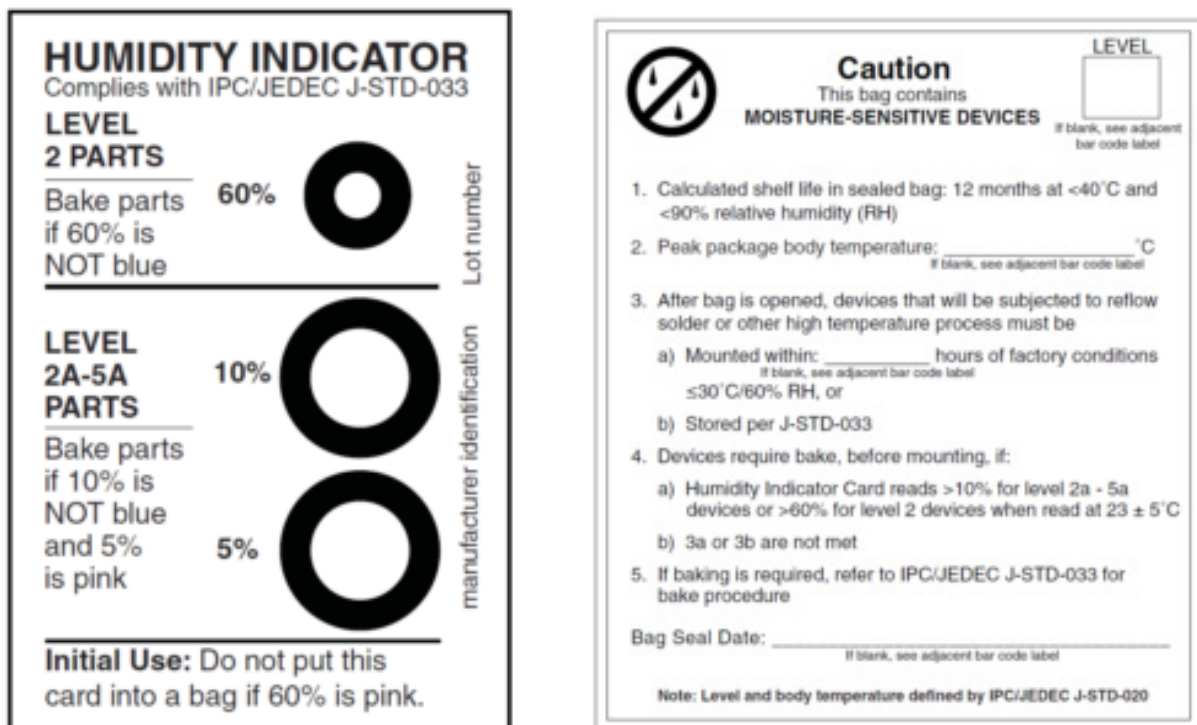
Figure 8: Example of humidity indicator and caution statement as per the J-STD-033C
