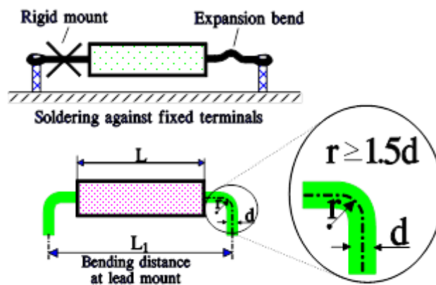
Figure 1: leaded components basic mounting rules, source: CLR HBK
