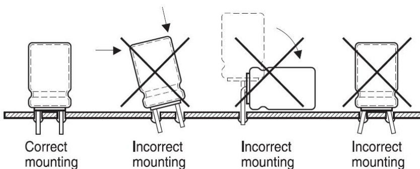
Figure 2: mounting considerations for single-ended capacitors, source: TDK
