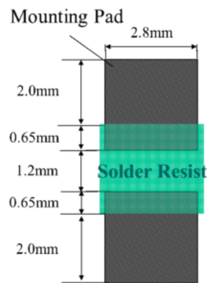
Figure 4: solder resist on a printed wiring board, source: Epectec*
