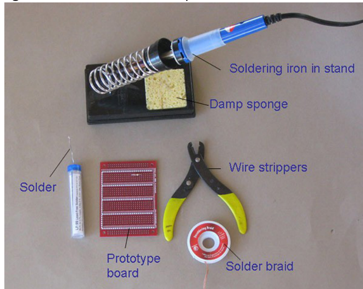
Figure 1. Soldering equipment and materials.
