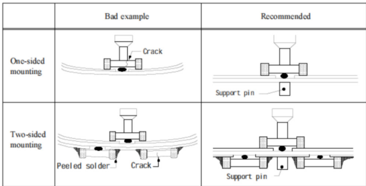
Figure 10: large board flex suppression by support pins, source: Kyocera
