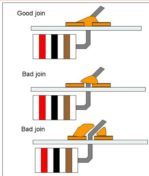
Figure 4. The solder in a good join will be shaped like a cone, with solid contact between the solder and all surfaces to be joined. Bad joins (also called dry joints) should be melted and remade.
