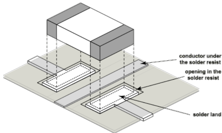
Figure 4: solder resist on a printed wiring board, source: Epectec*
