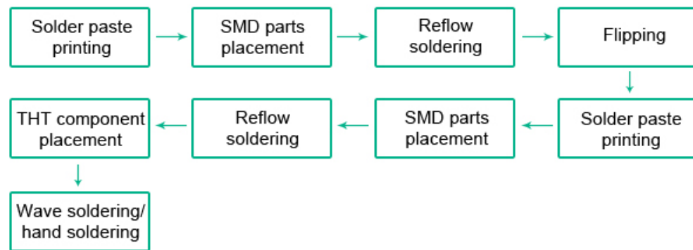
Figure 7 Double side Mixed Assembly Workflow (2)
