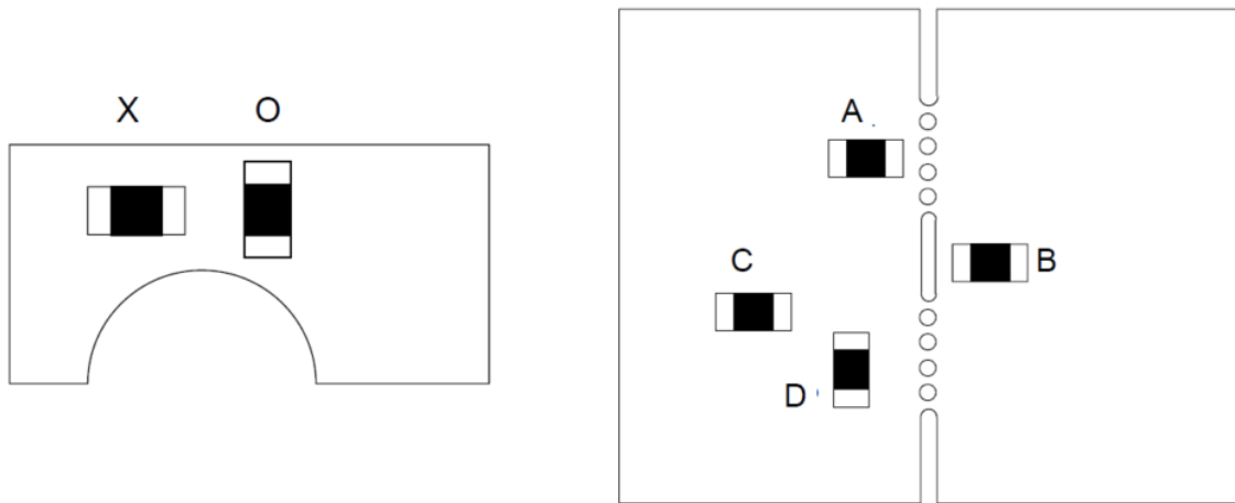
Figure 7: SMD component arrangement close to curvature, bending or PCB crop lines. Source: Panasonic
