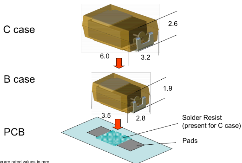
Figure 5: tantalum capacitors C to B case universal pad design source: AVX
