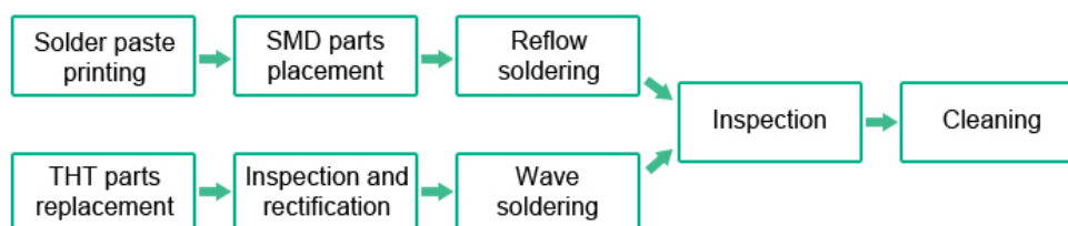
Figure 3 Procedure Comparison between SMT Assembly and THT Assembly
